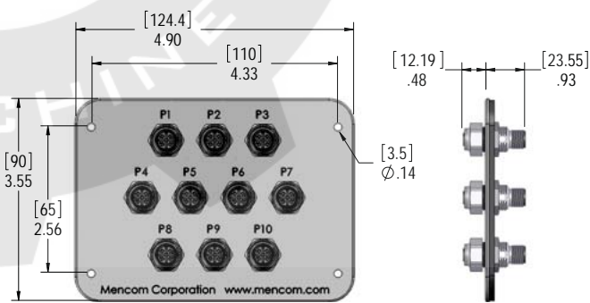
10 Port Version
