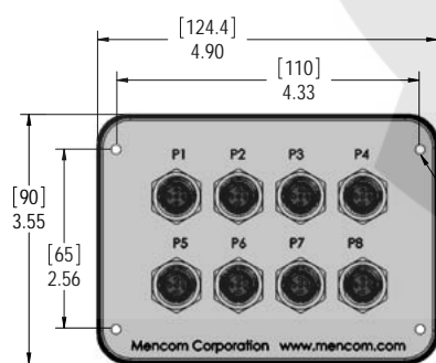
8 Port Version
