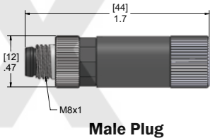
Male Plug
