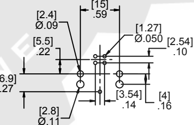
4 Pole Female Right angle Layout
