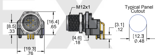
Male Right Angle
