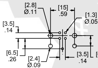
4 Pole Male Straight Layout
