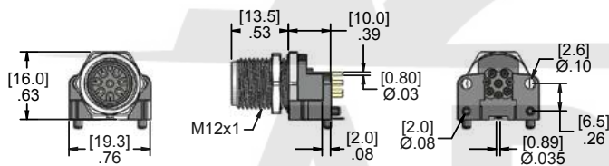
Male Straight
