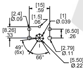
Straight Layout
