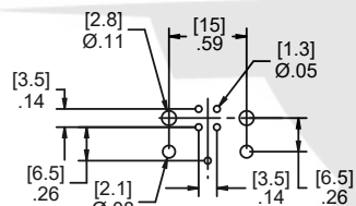
4 Pole Male Straight Layout
