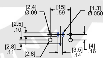
4 Pole Male Right Angle Layout
