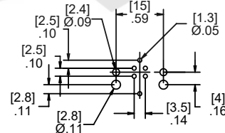
5 Pole Male Right Angle Layout
