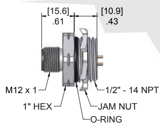
Male Receptacles
