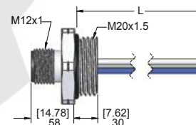
Male Receptacle
