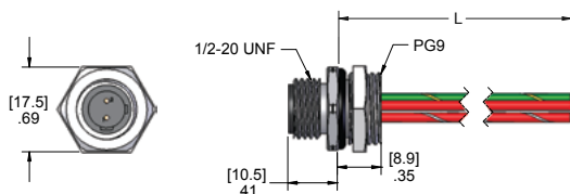
PG9 Threads
