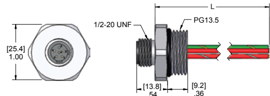
PG13.5 Threads
