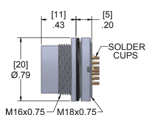
Male Receptacle
