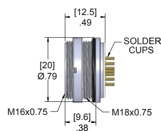
Female Receptacle
