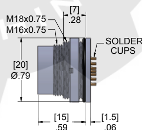
Male Receptacle
