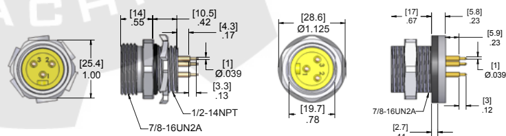
Male Front Mount Receptacle
