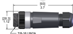
Male Straight (Male Threads)
