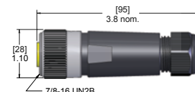
Female Straight (Female Threads)
