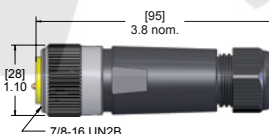
Male Straight (Female Threads)
