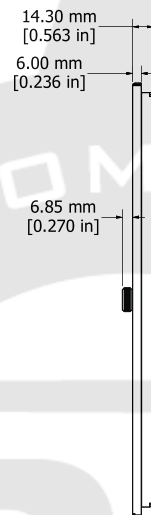
ASSEMBLY - VIEW FROM SIDE
