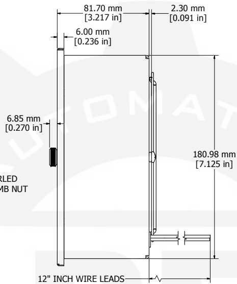
ASSEMBLY - VIEW FROM SIDE
