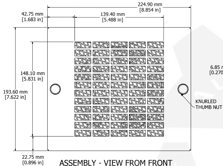
ASSEMBLY - VIEW FROM FRONT
