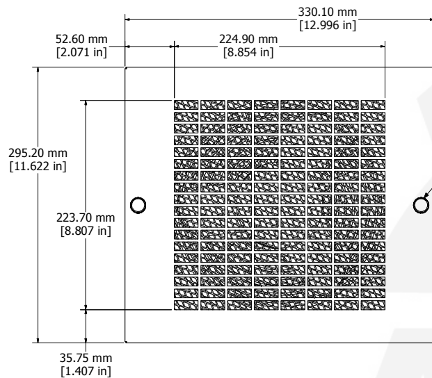
ASSEMBLY - VIEW FROM FRONT
