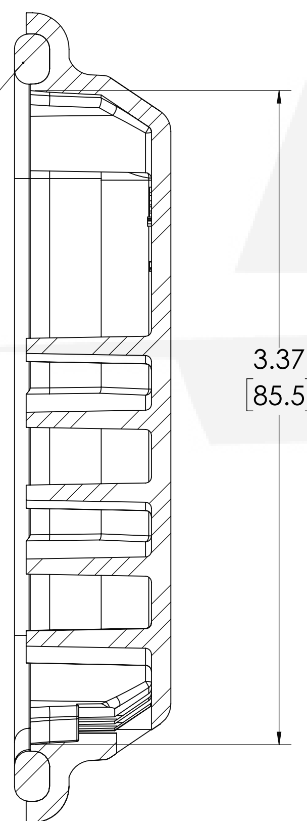
SECTION B-B
