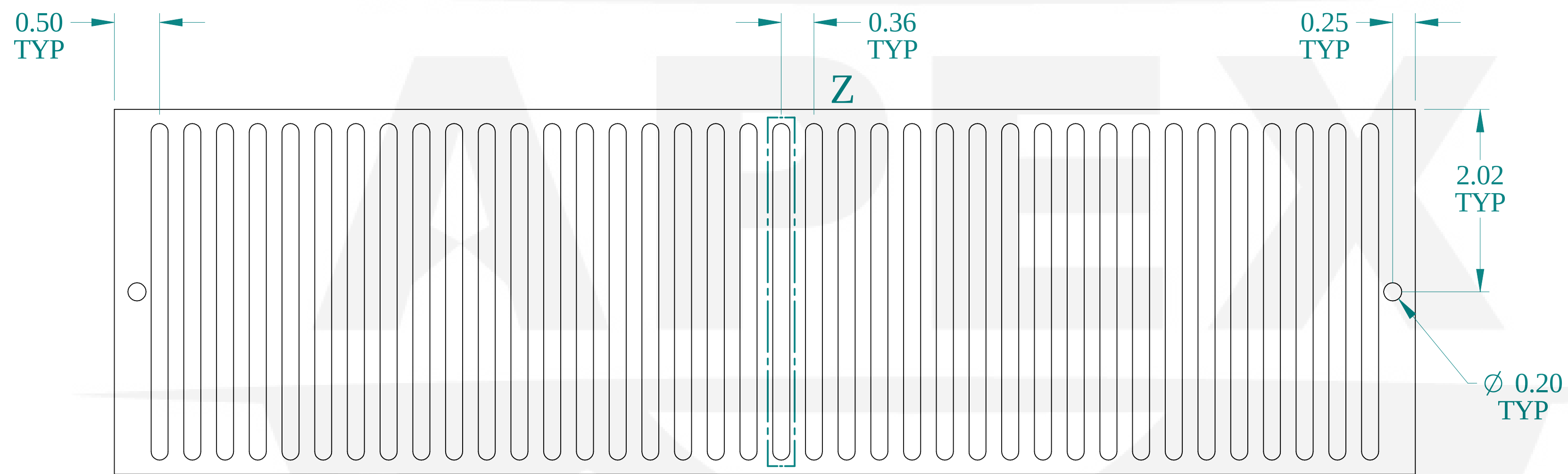
FRONT VIEW
