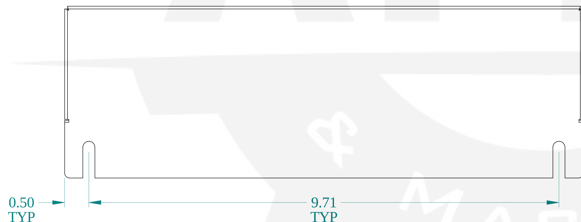
FRONT VIEW
