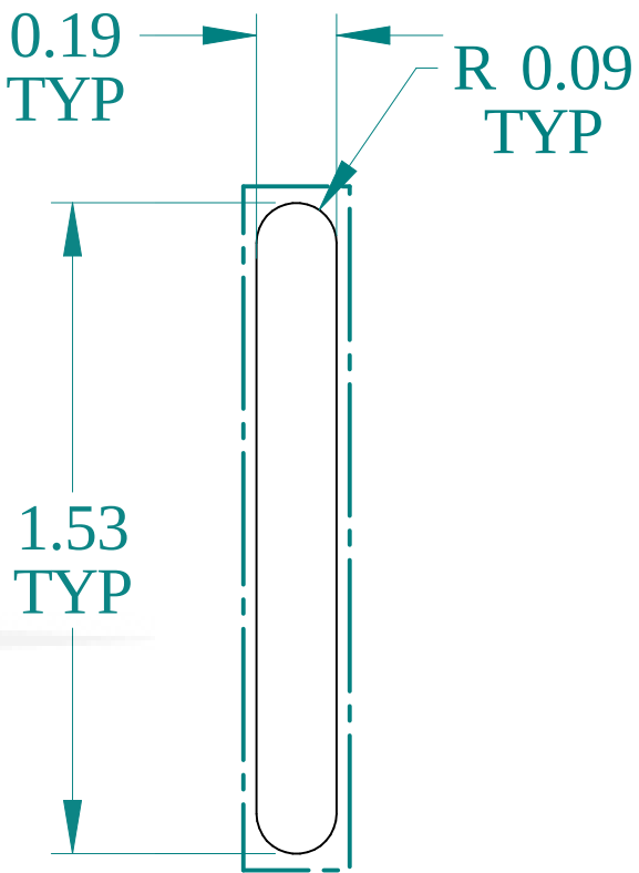
DETAIL Z
