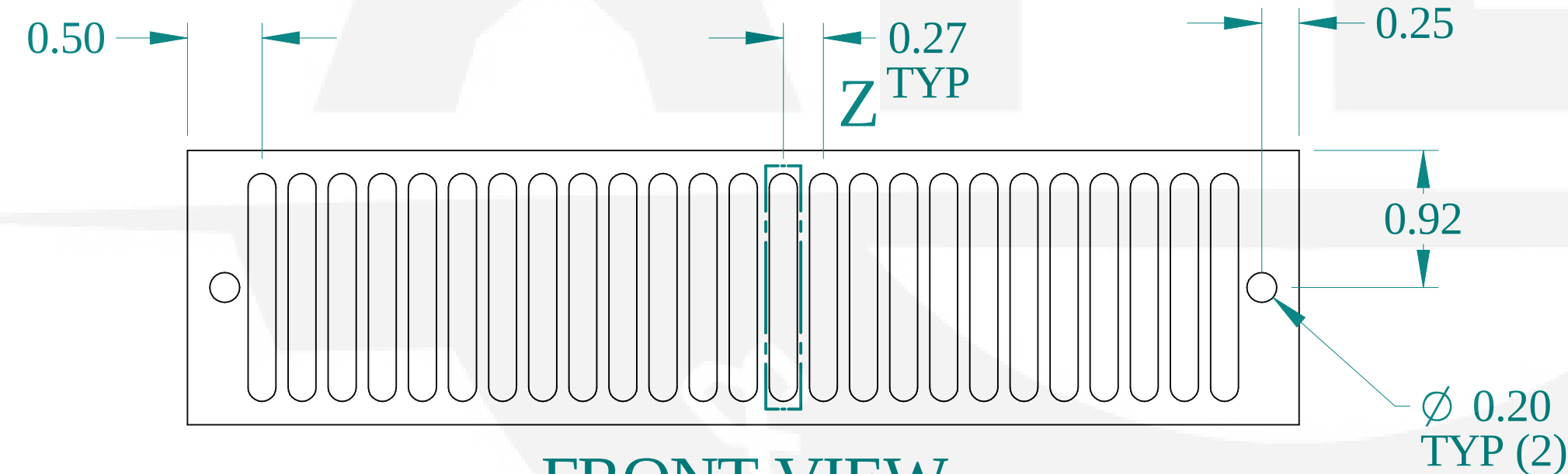
FRONT VIEW
