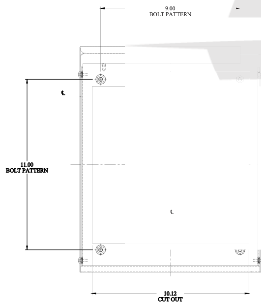
BACK VIEW
