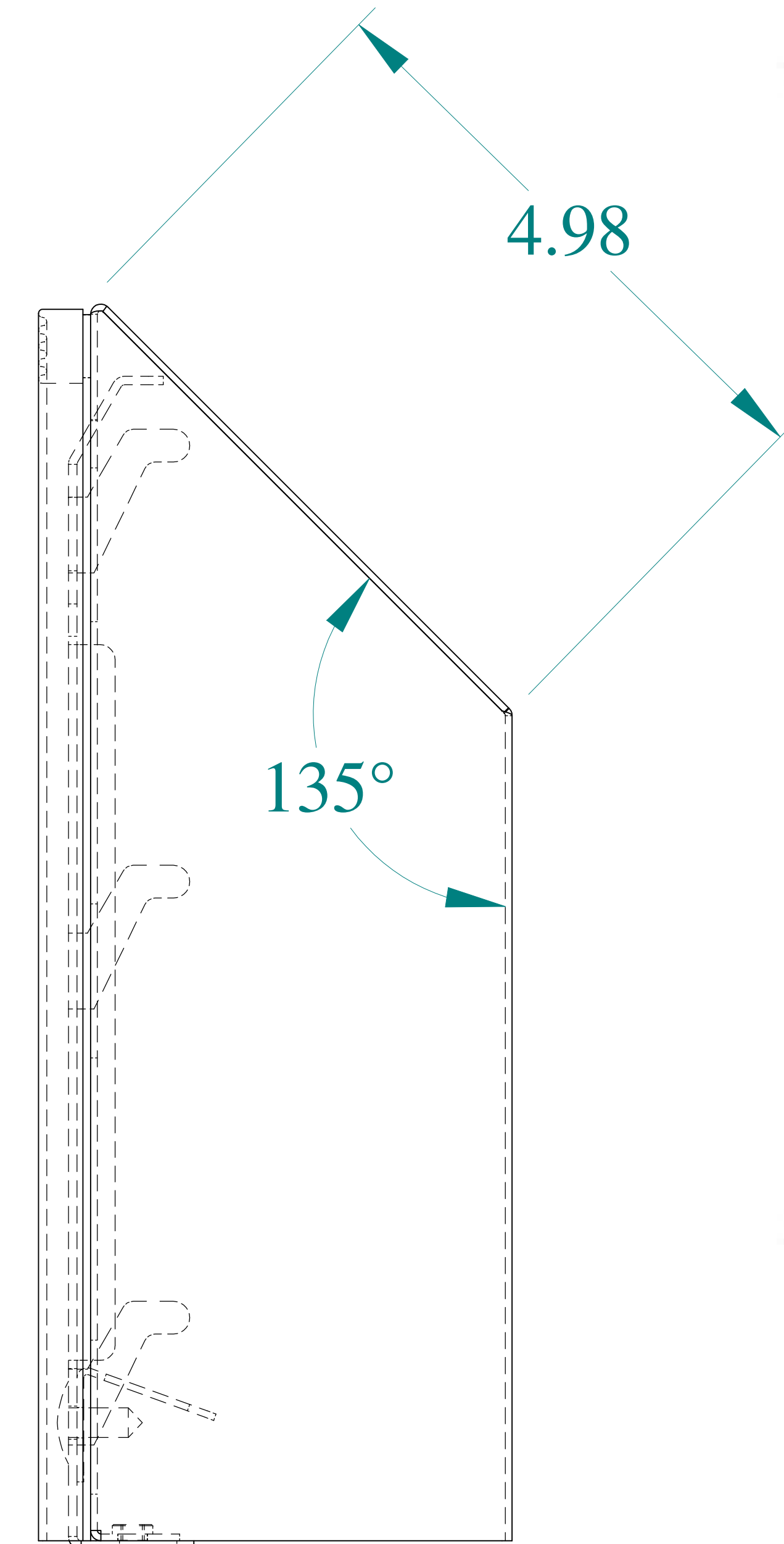
SIDE VIEW
