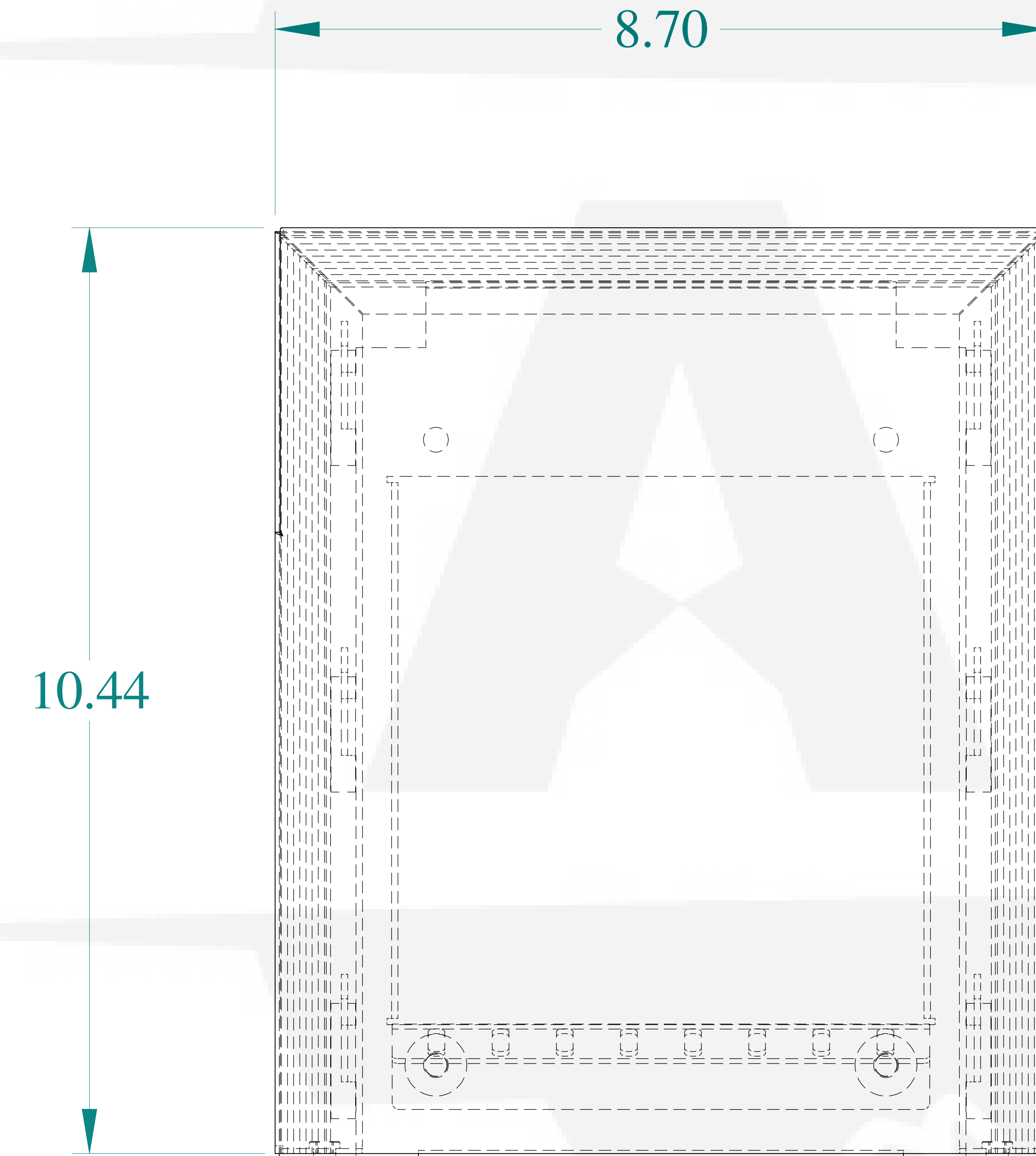
FRONT VIEW
