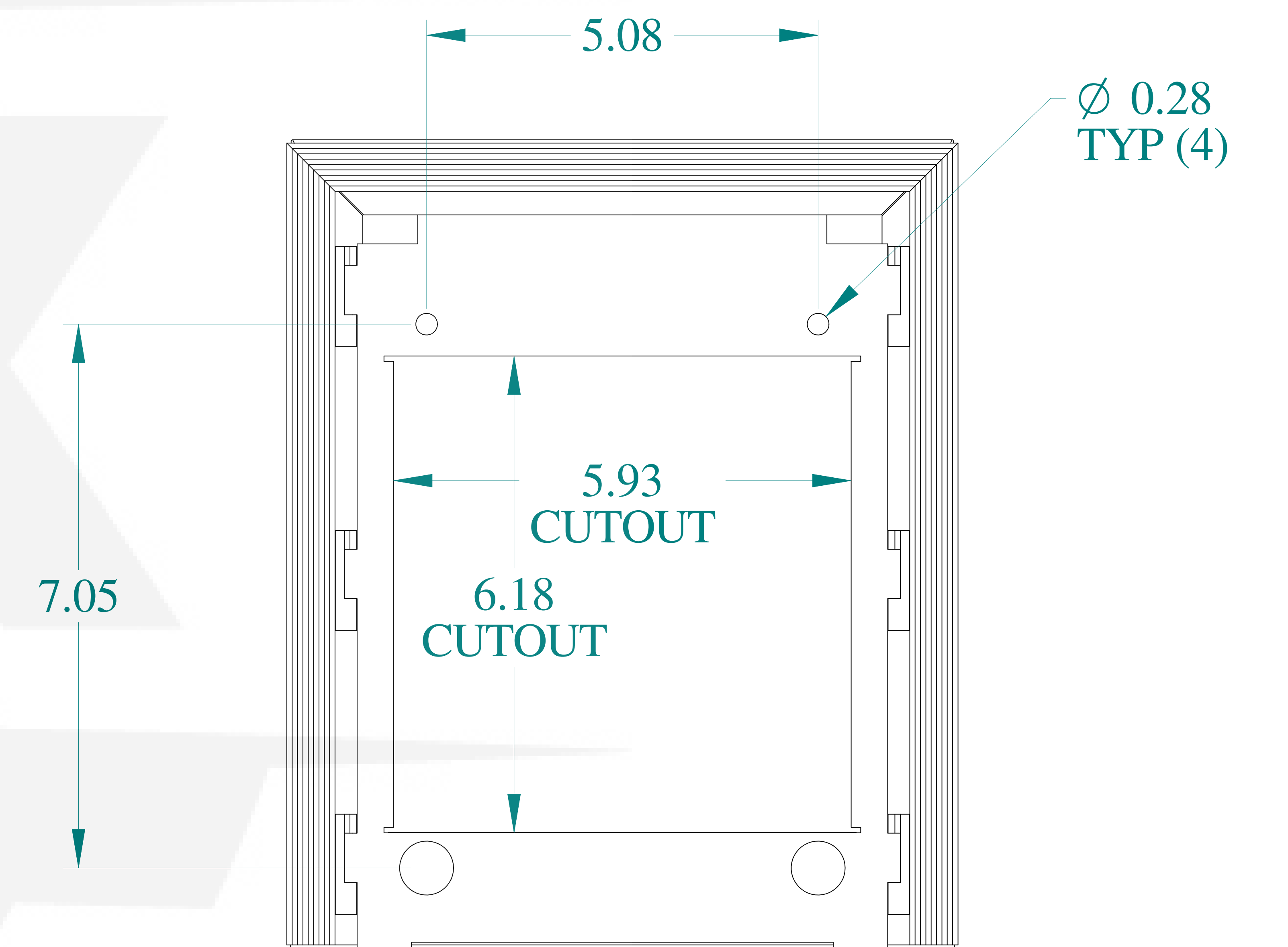
BACK VIEW
