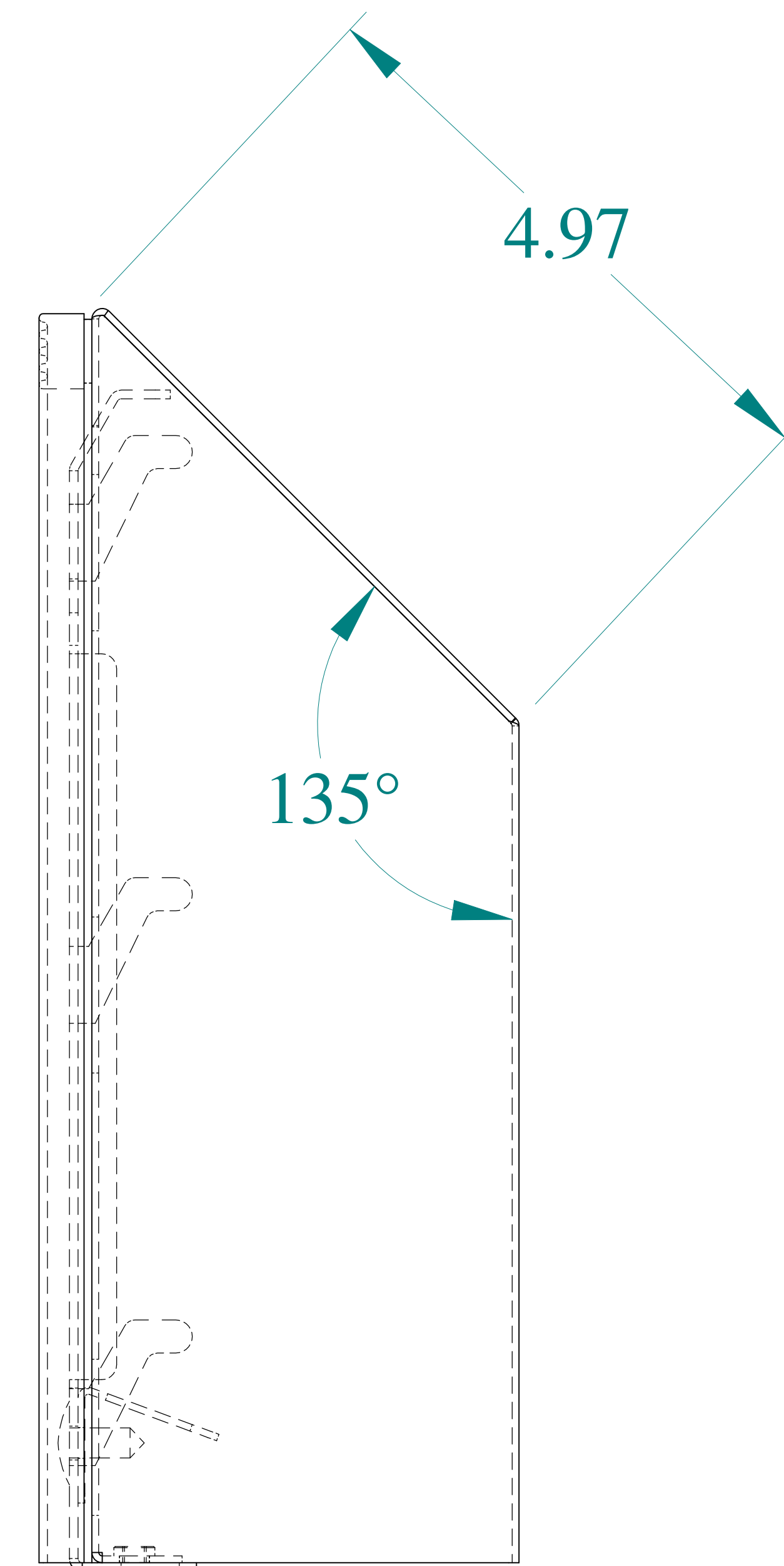
SIDE VIEW
