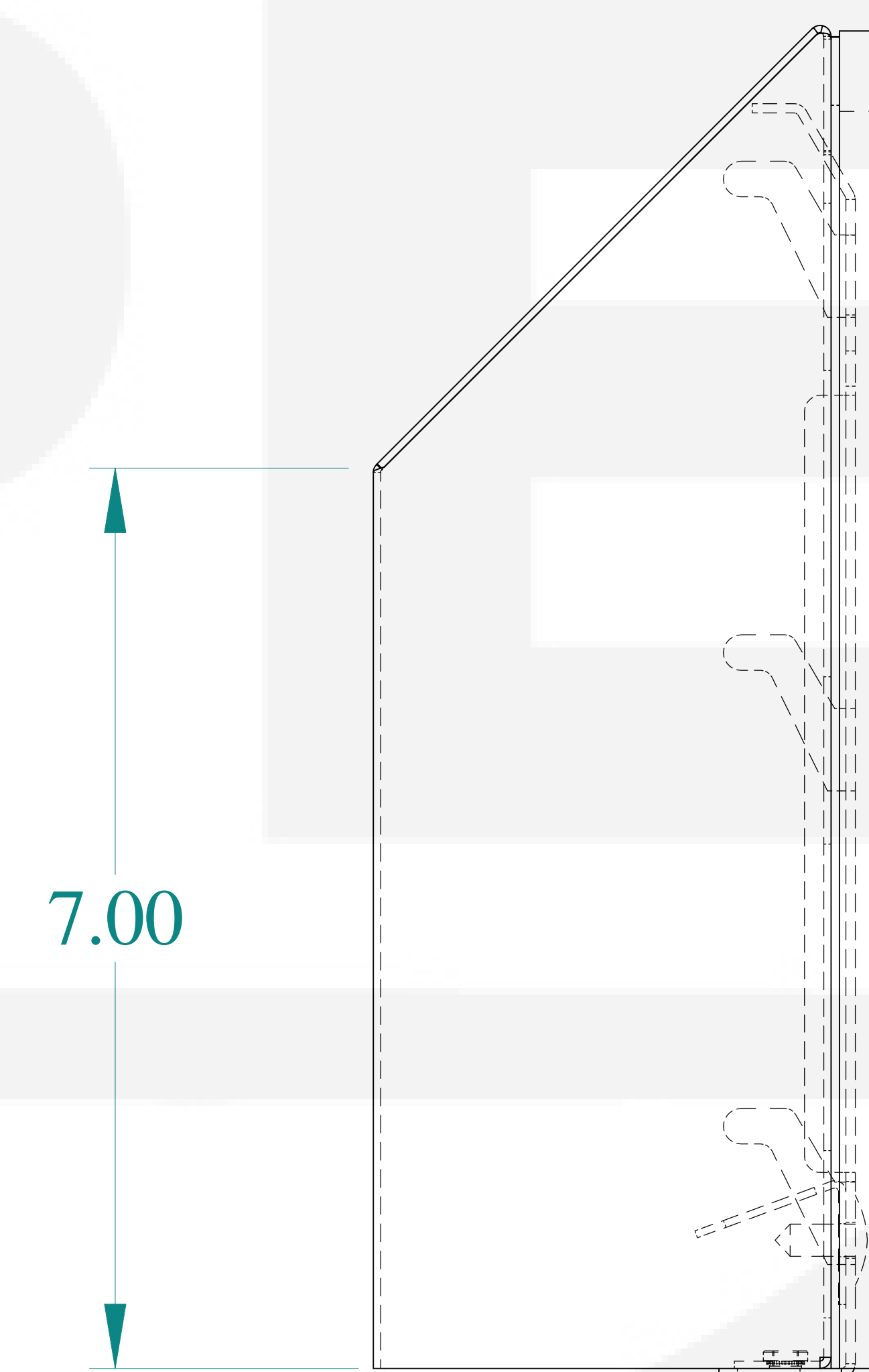
SIDE VIEW
