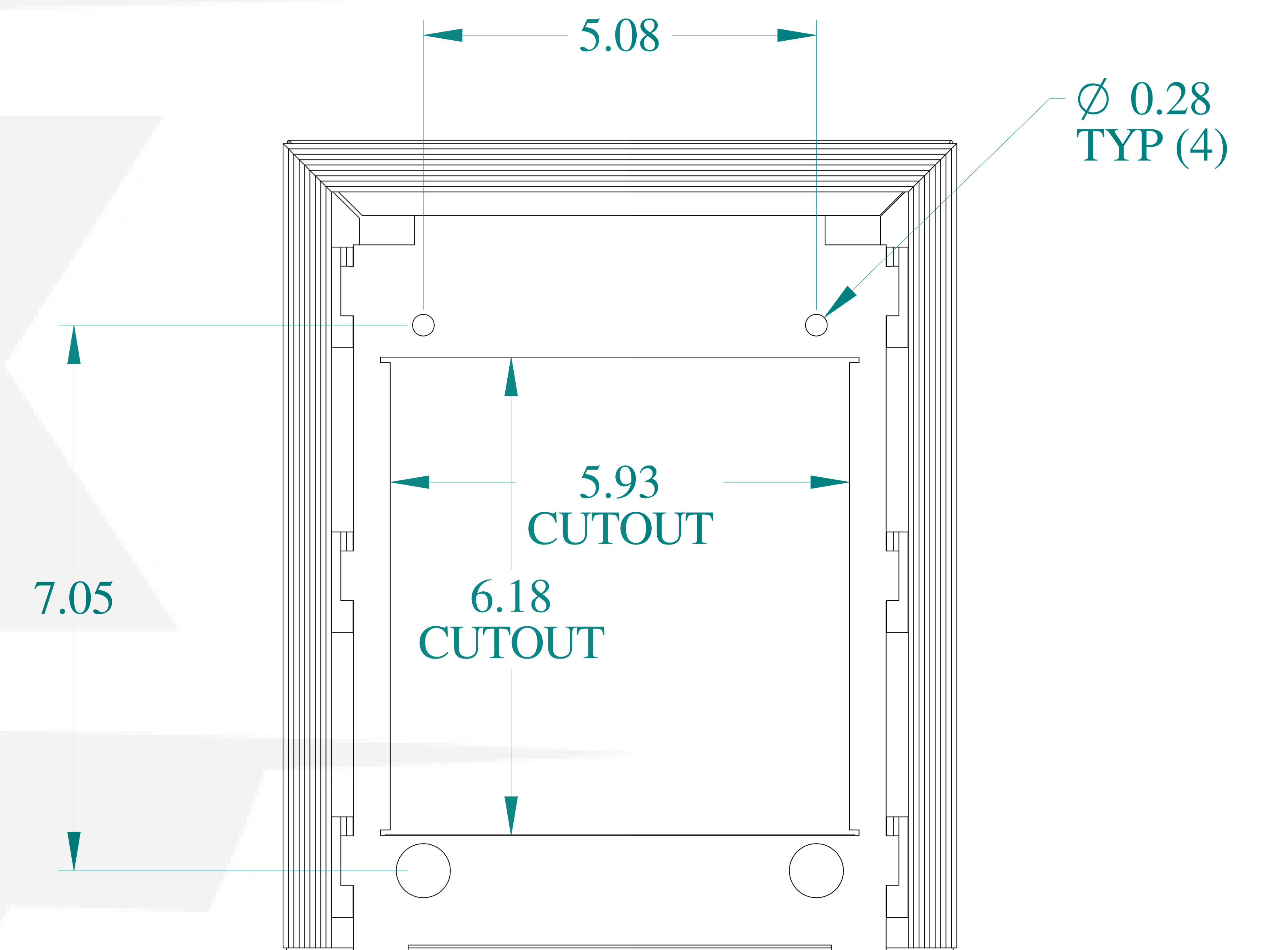
BACK VIEW
