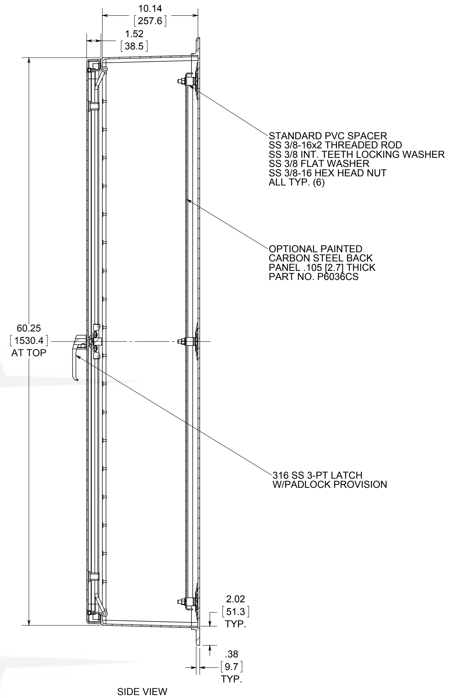
SIDE VIEW
