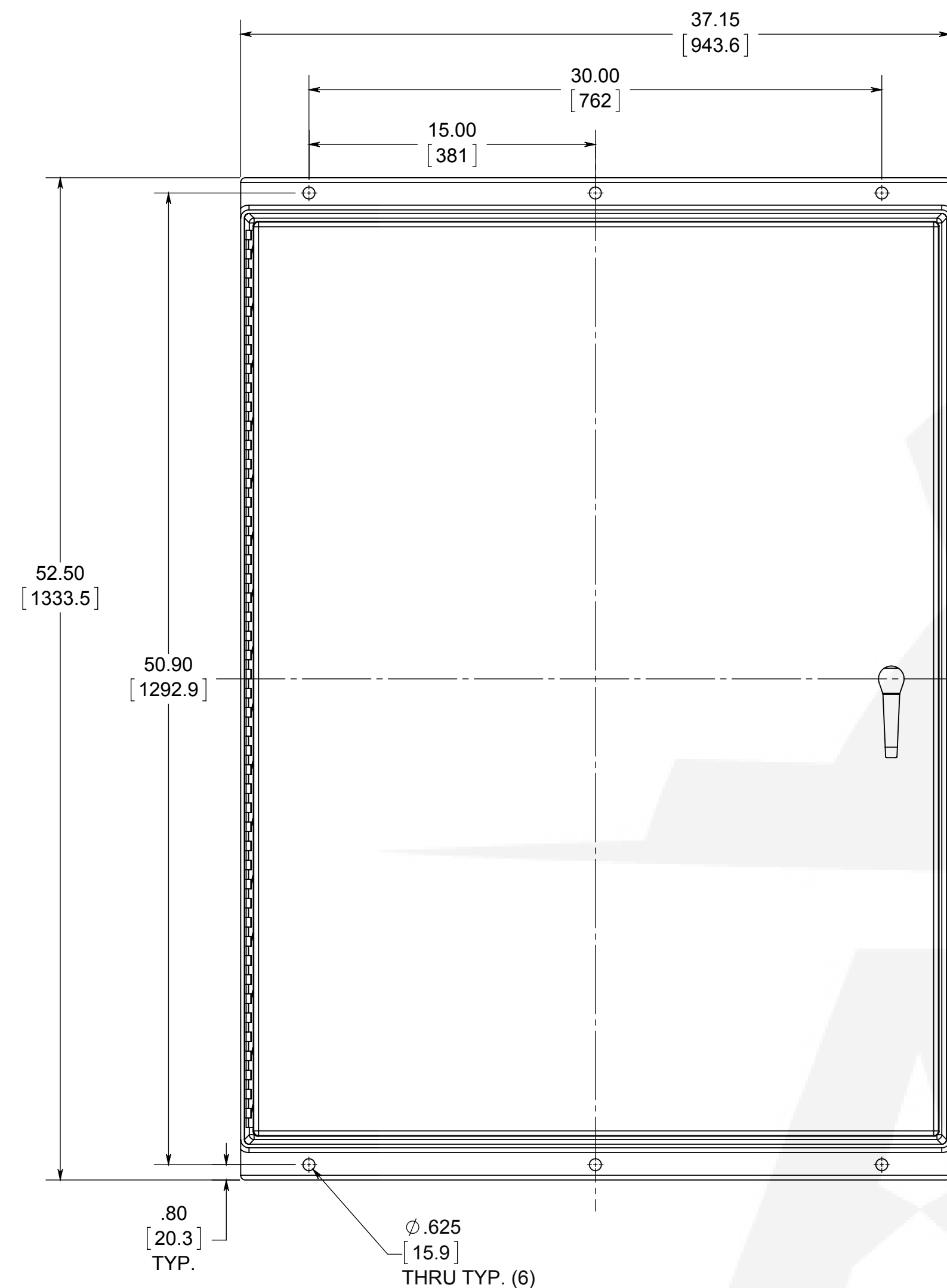
FRONT VIEW WITH COVER
