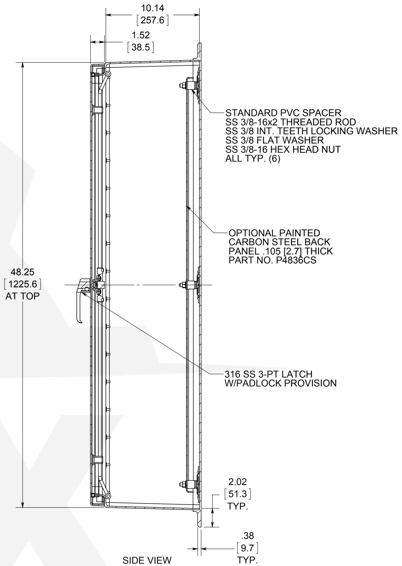
SIDE VIEW
