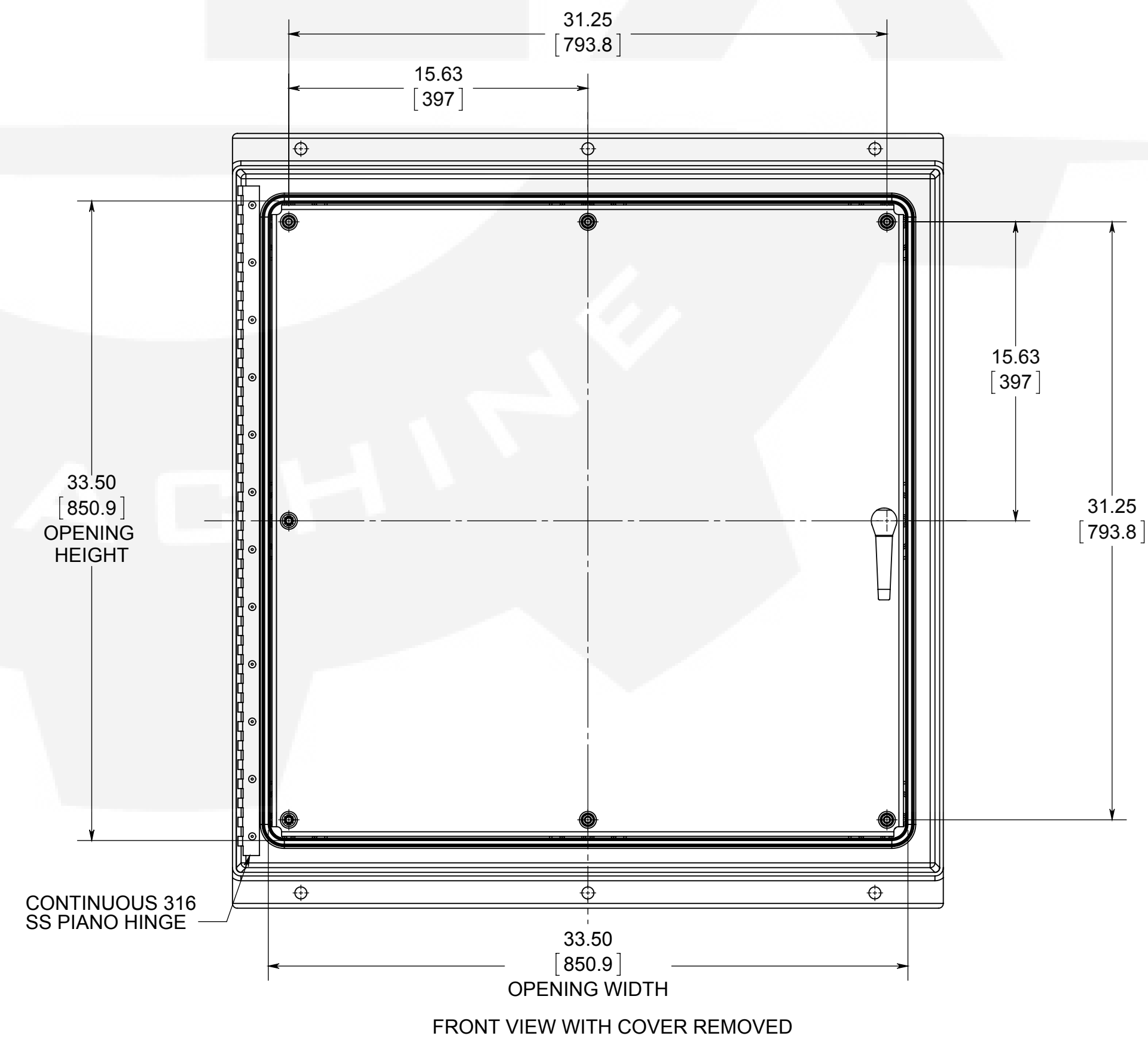
FRONT VIEW WITH COVER REMOVED
