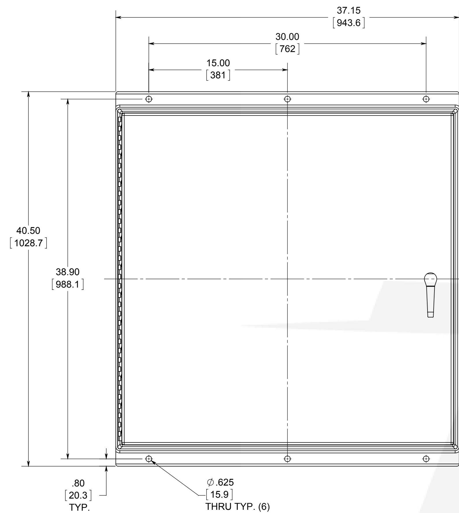
FRONT VIEW WITH COVER
