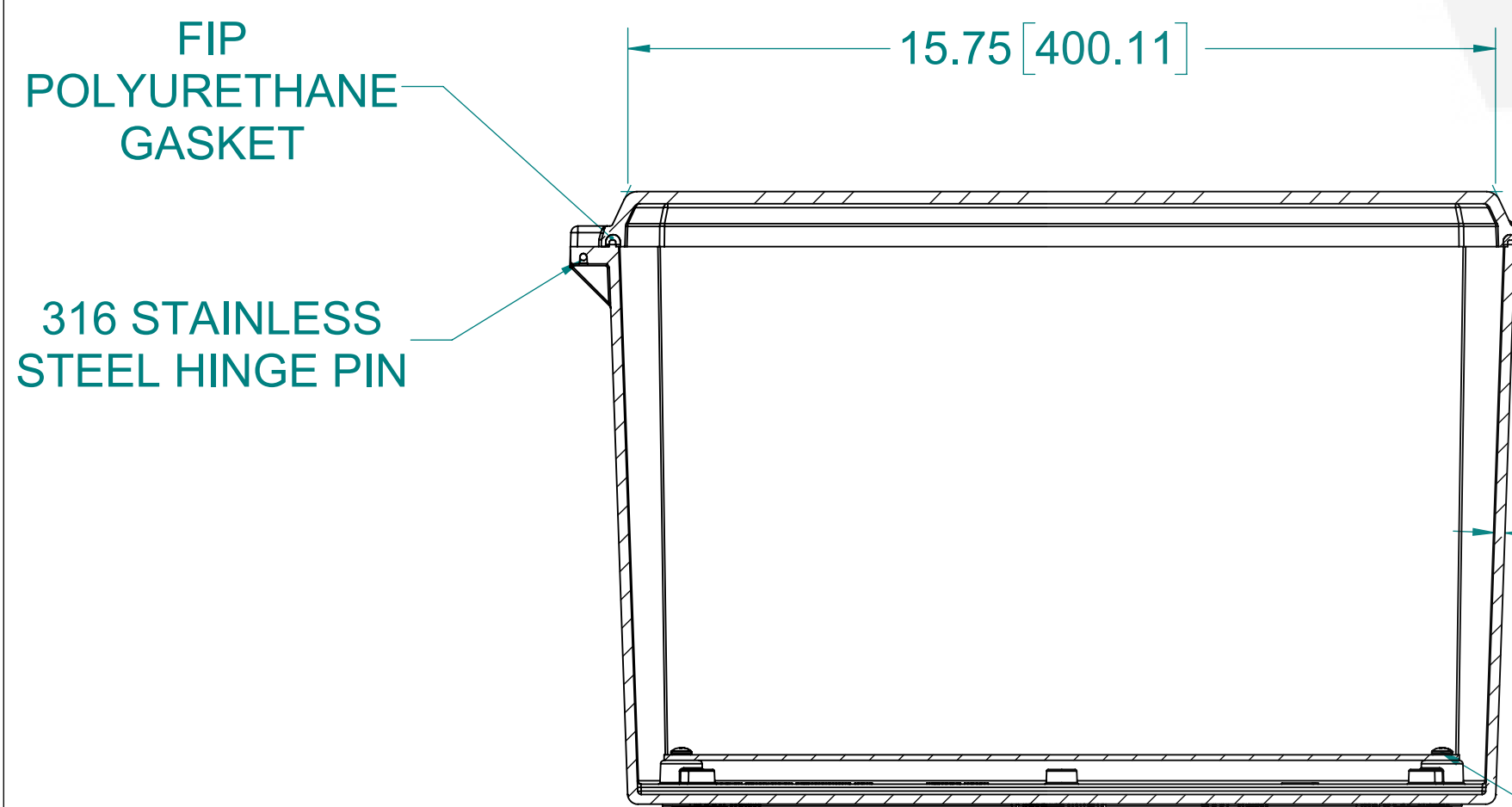
SECTION B-B
