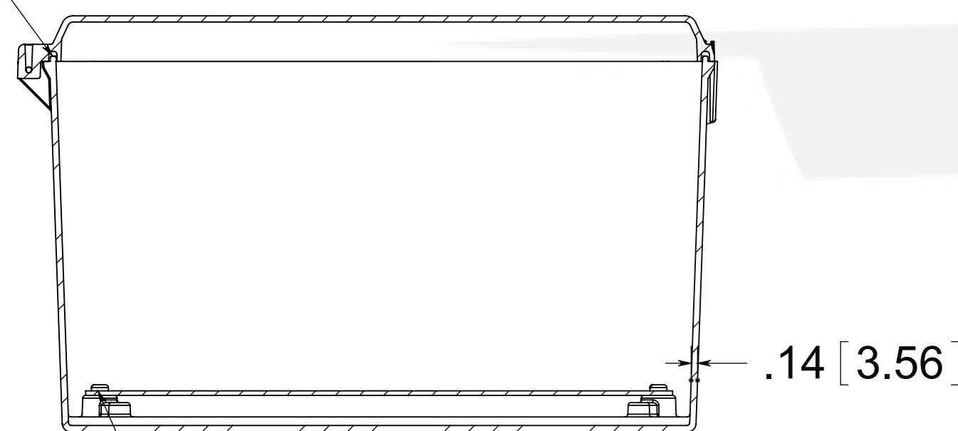
SECTION B-B
