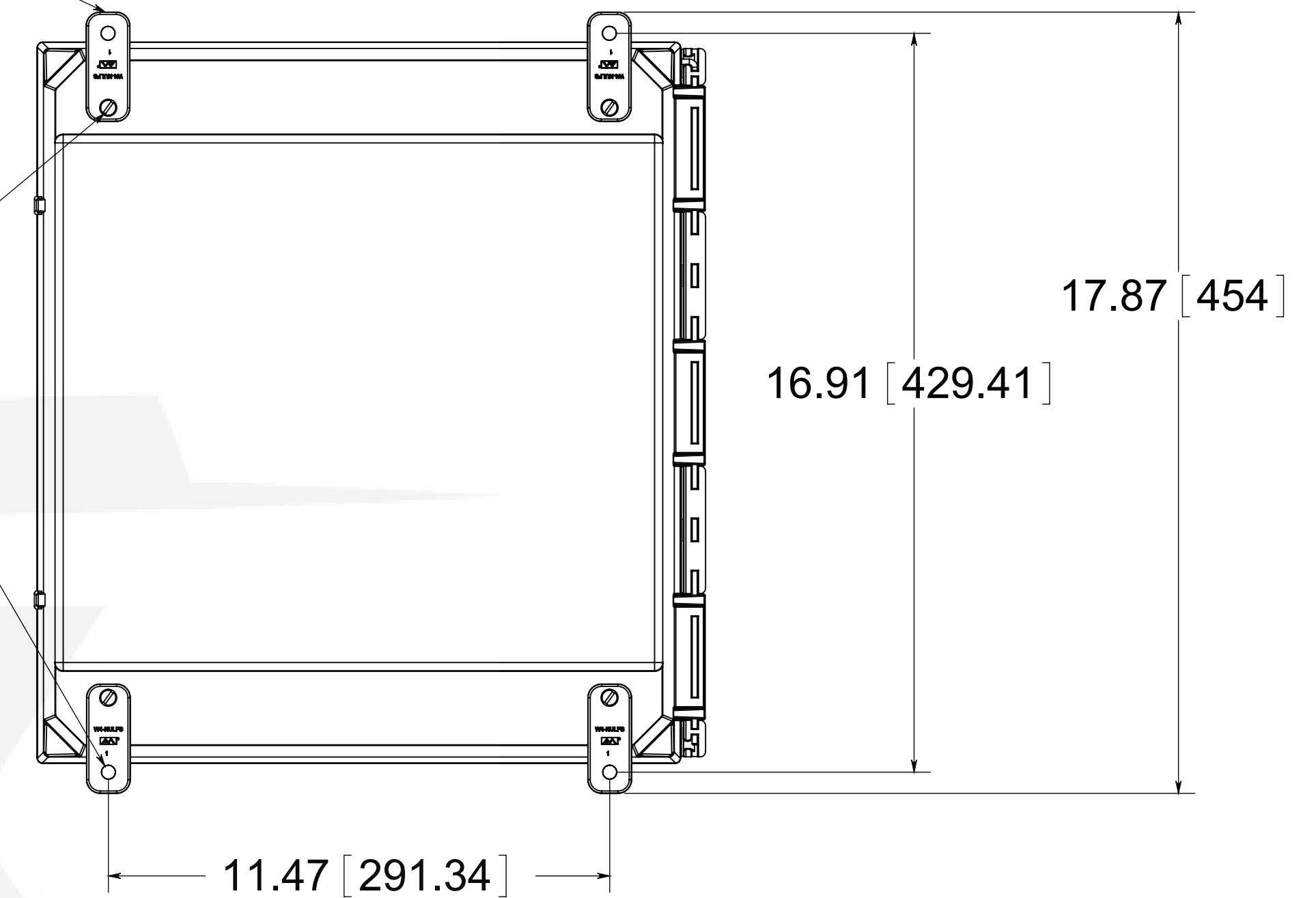
BACK VIEW
