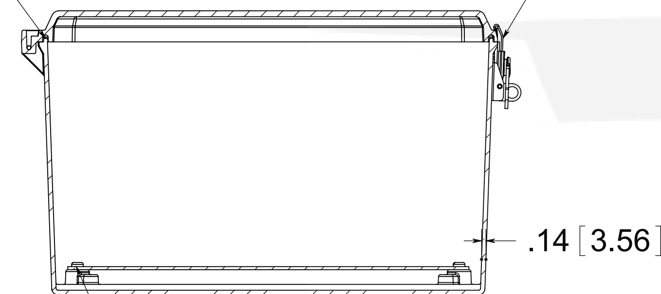
SECTION B-B
