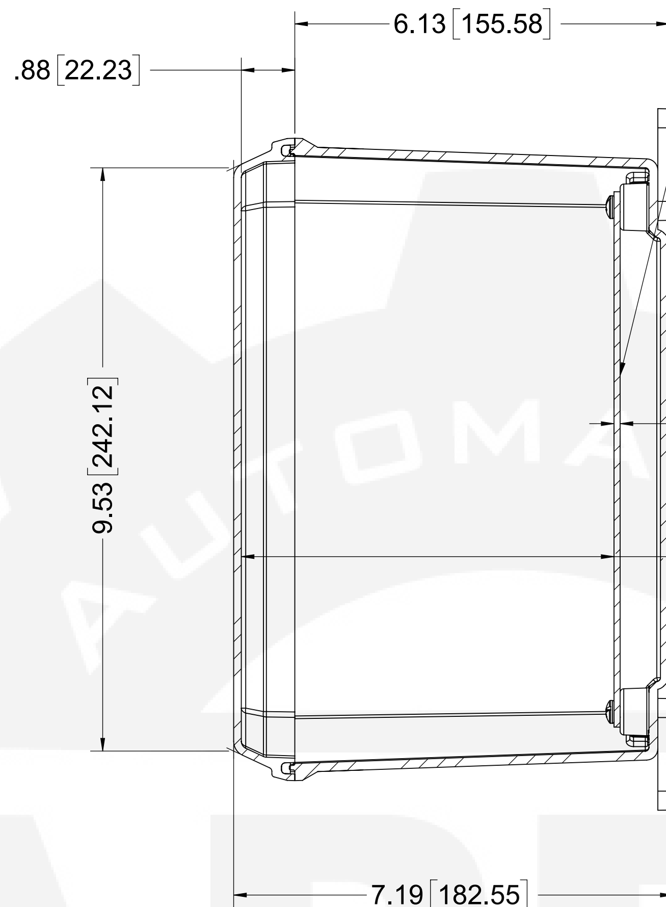
SECTION B-B
