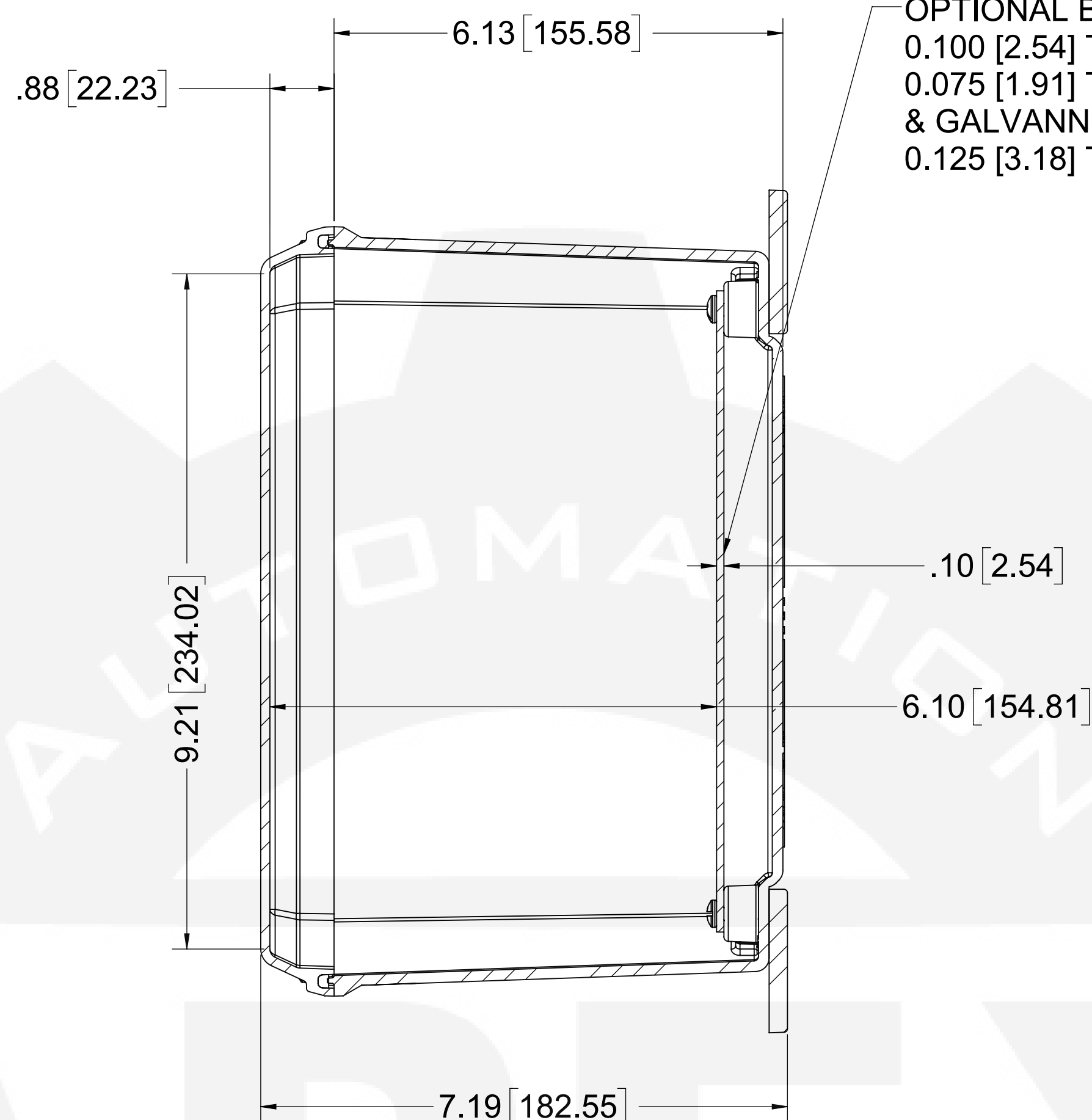
SECTION B-B
