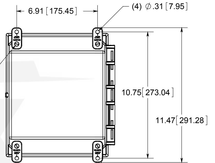
BACK VIEW
