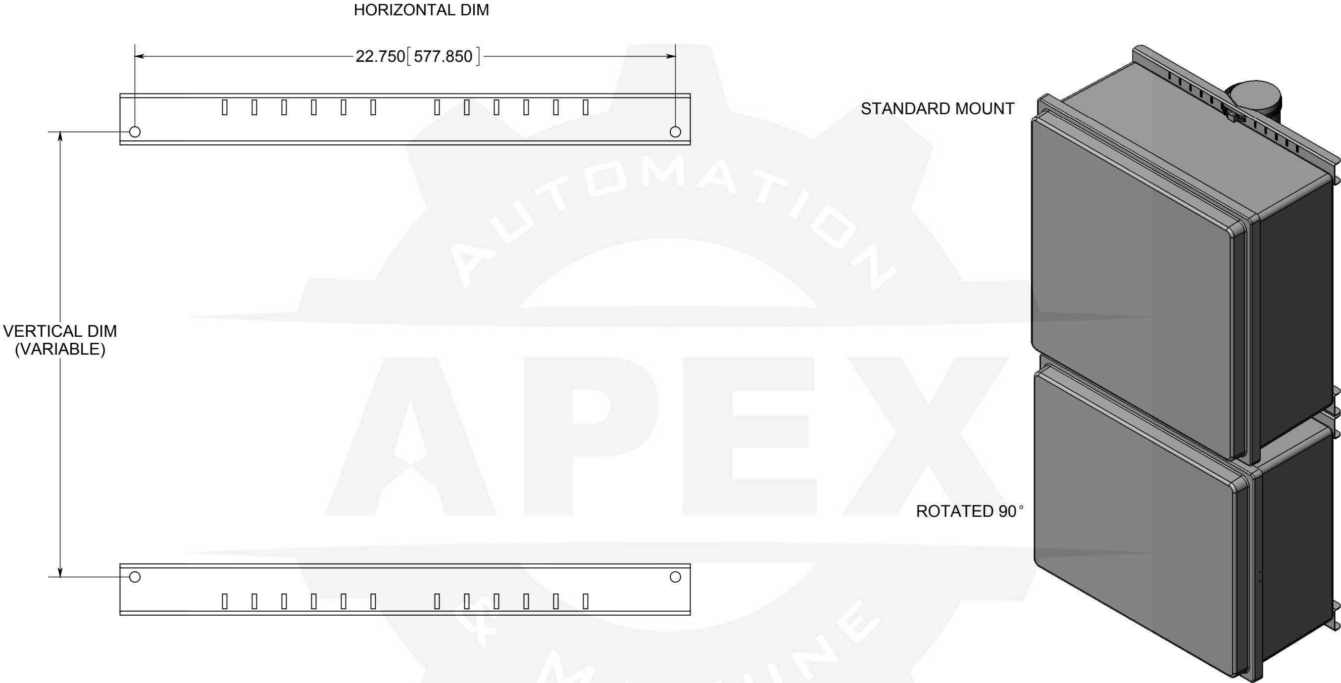
STANDARD MOUNT HOLE PATTERN
