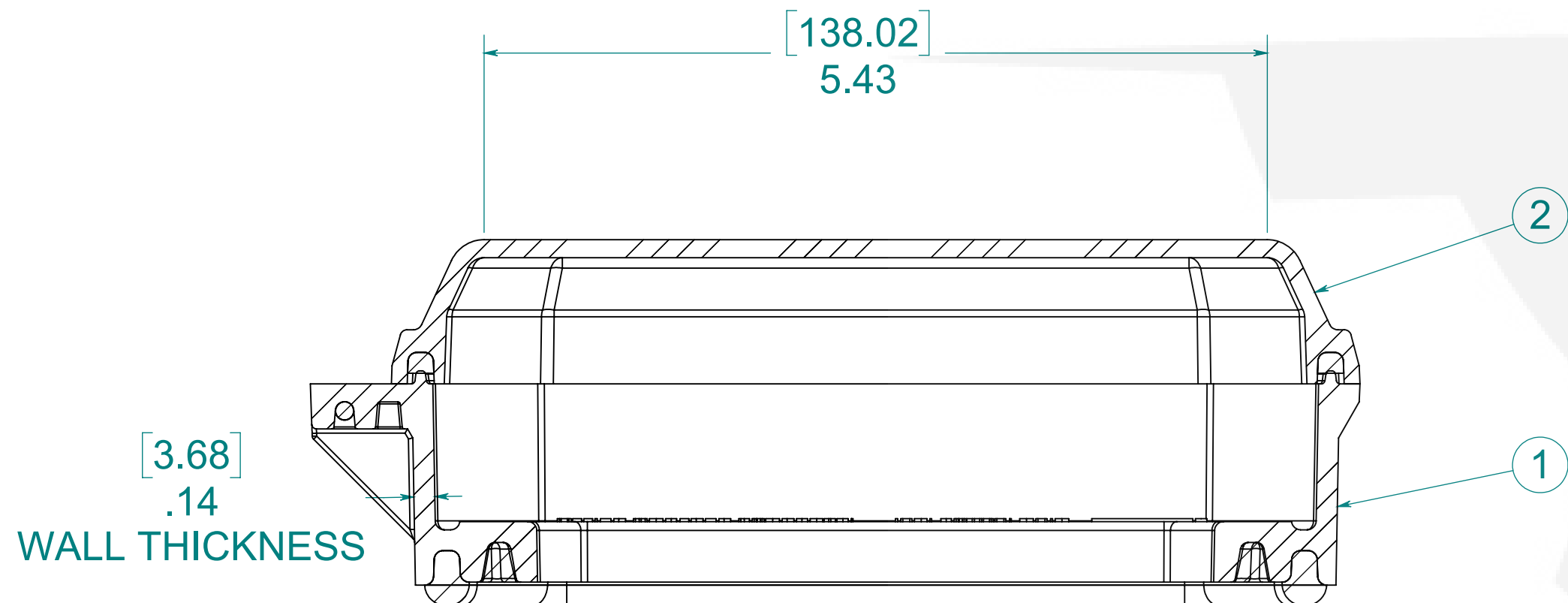
SECTION B-B
