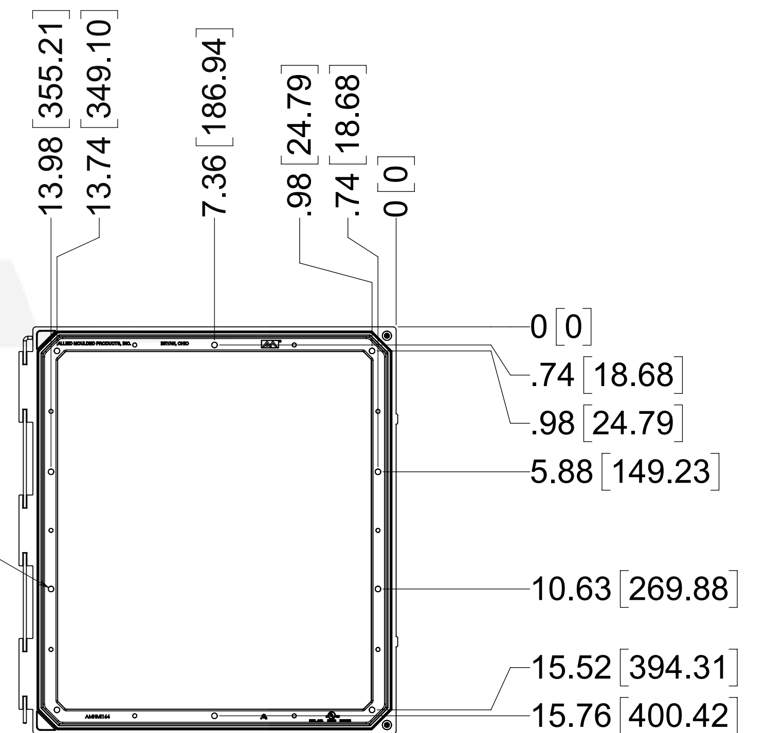
MOUNTING HOLE PATTERN HMI164
