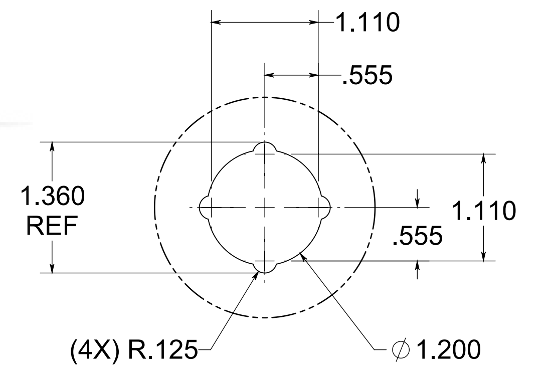
DETAIL D 30.5MM HOLE SCALE 1 : 1
