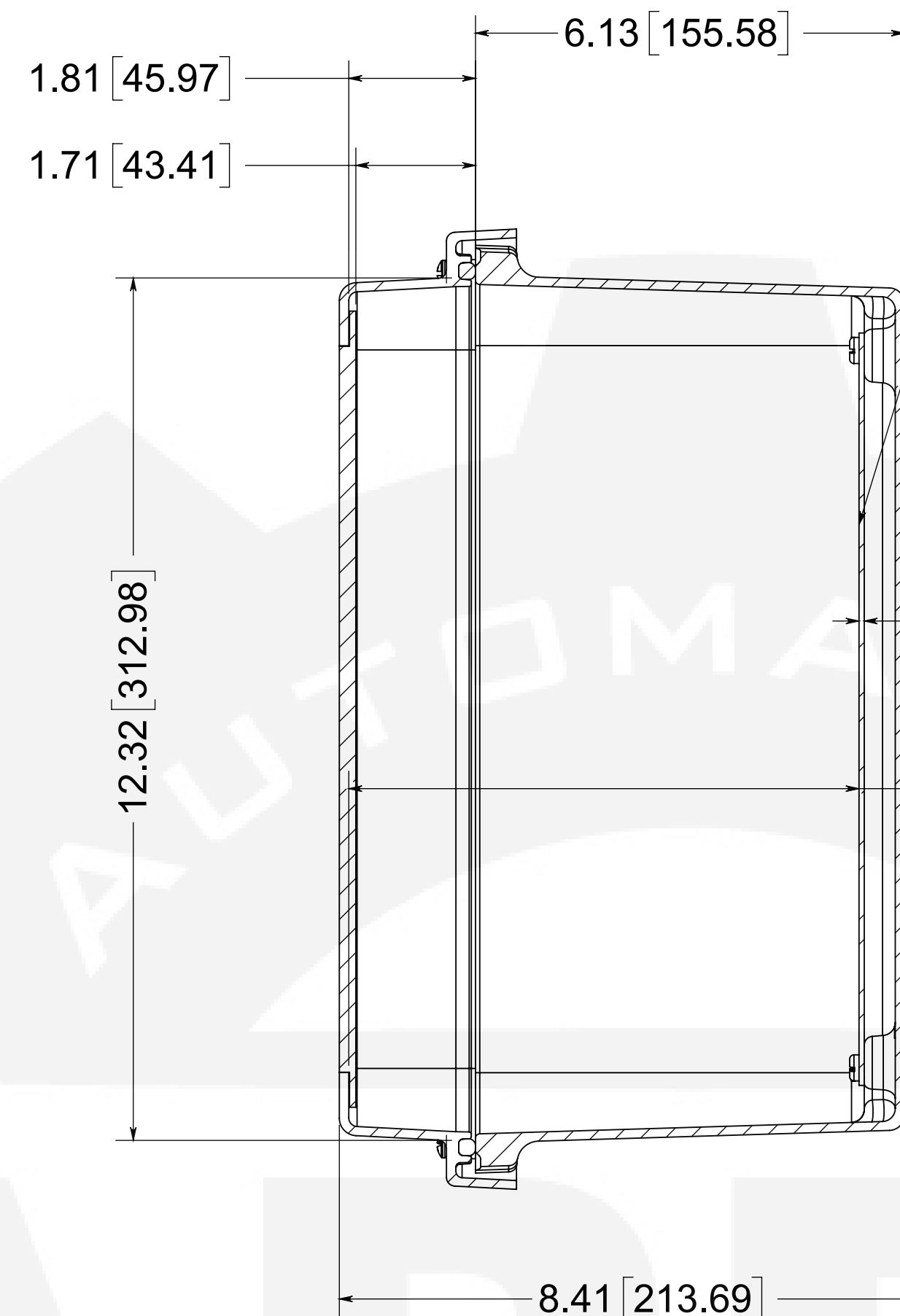
SECTION B-B
