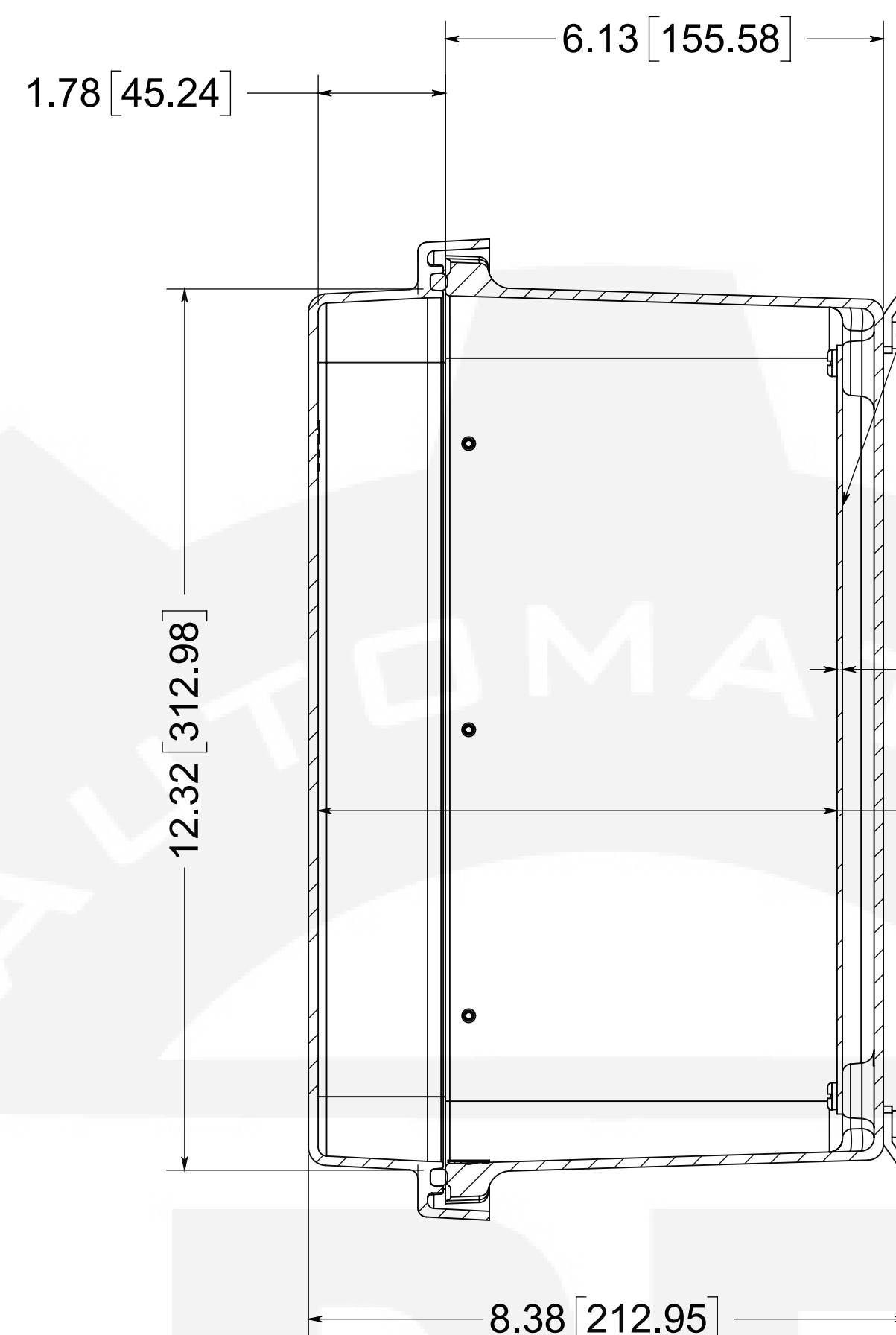
SECTION B-B
