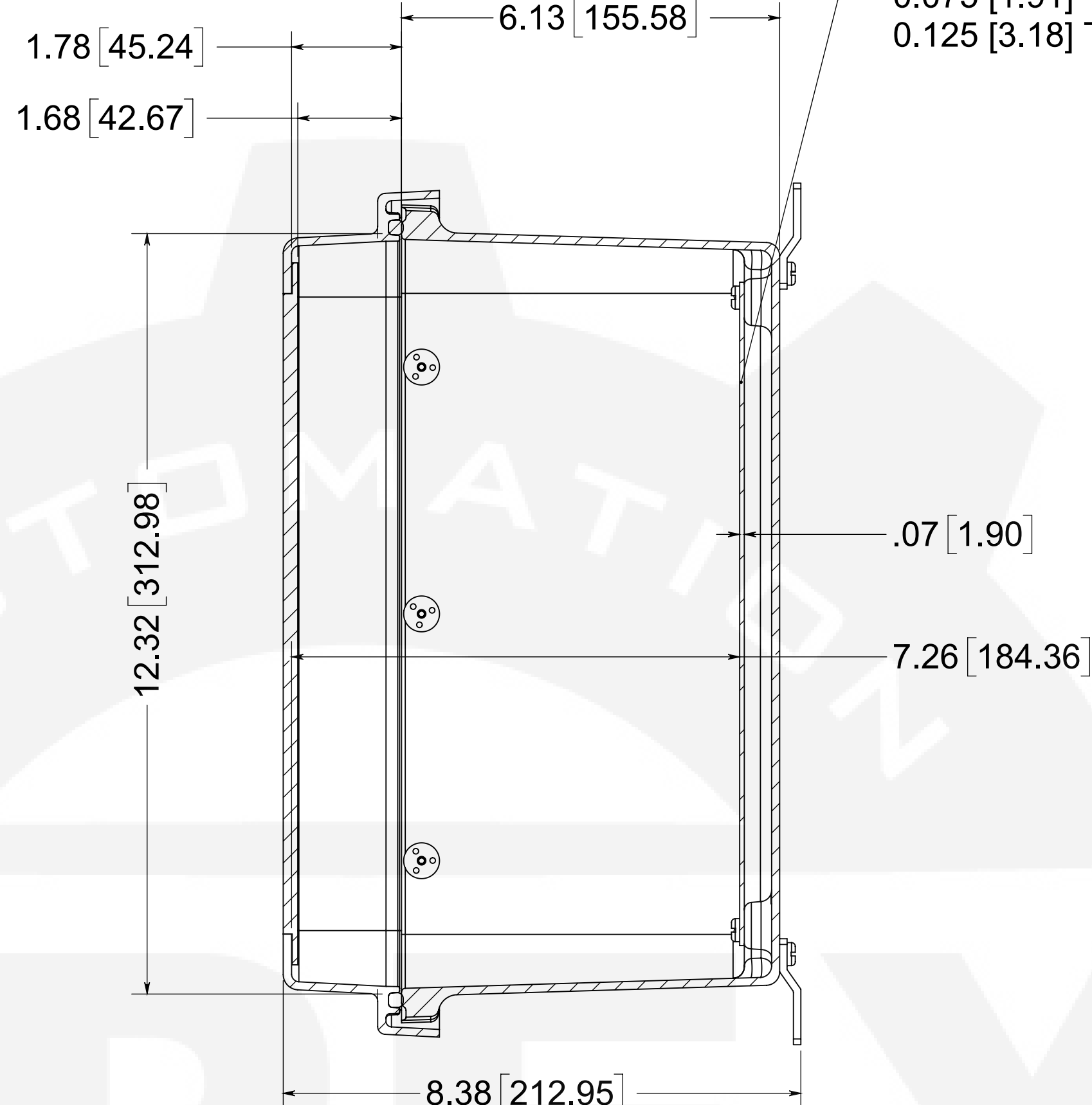
SECTION B-B
