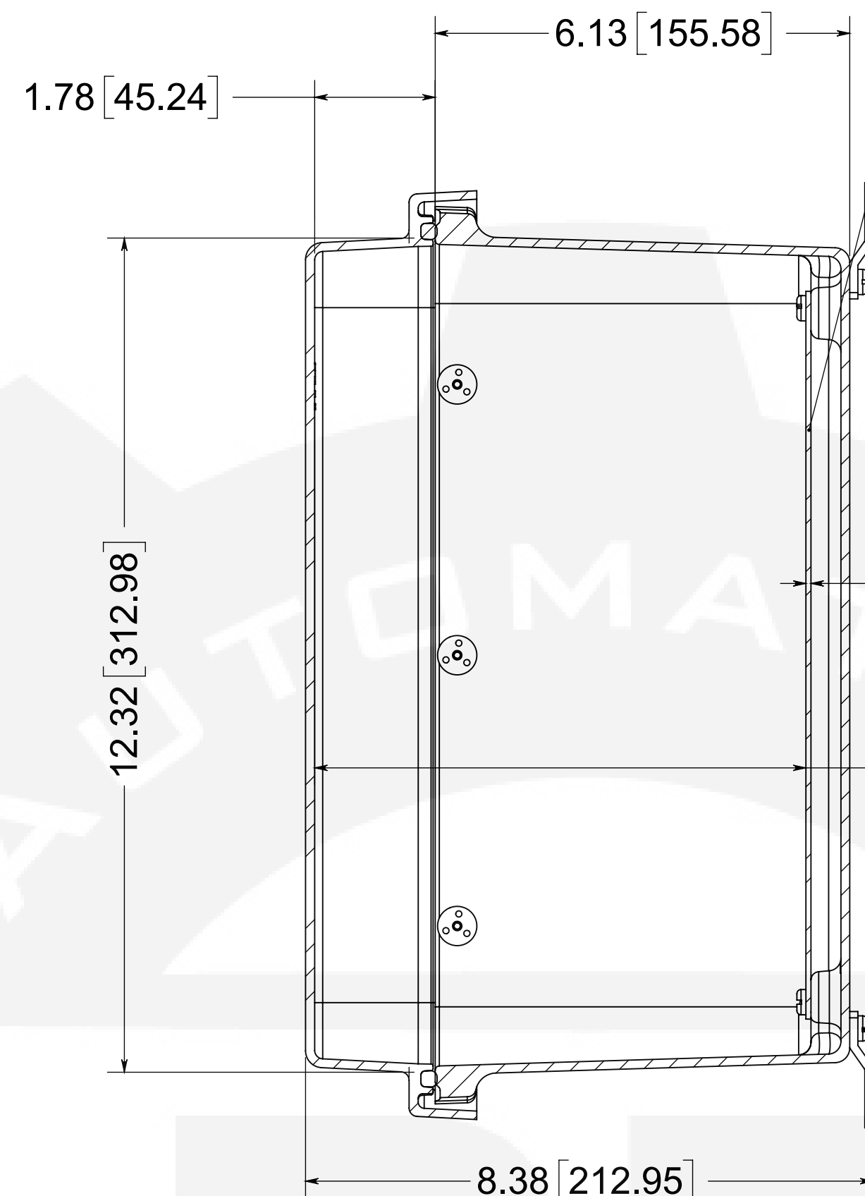
SECTION B-B
