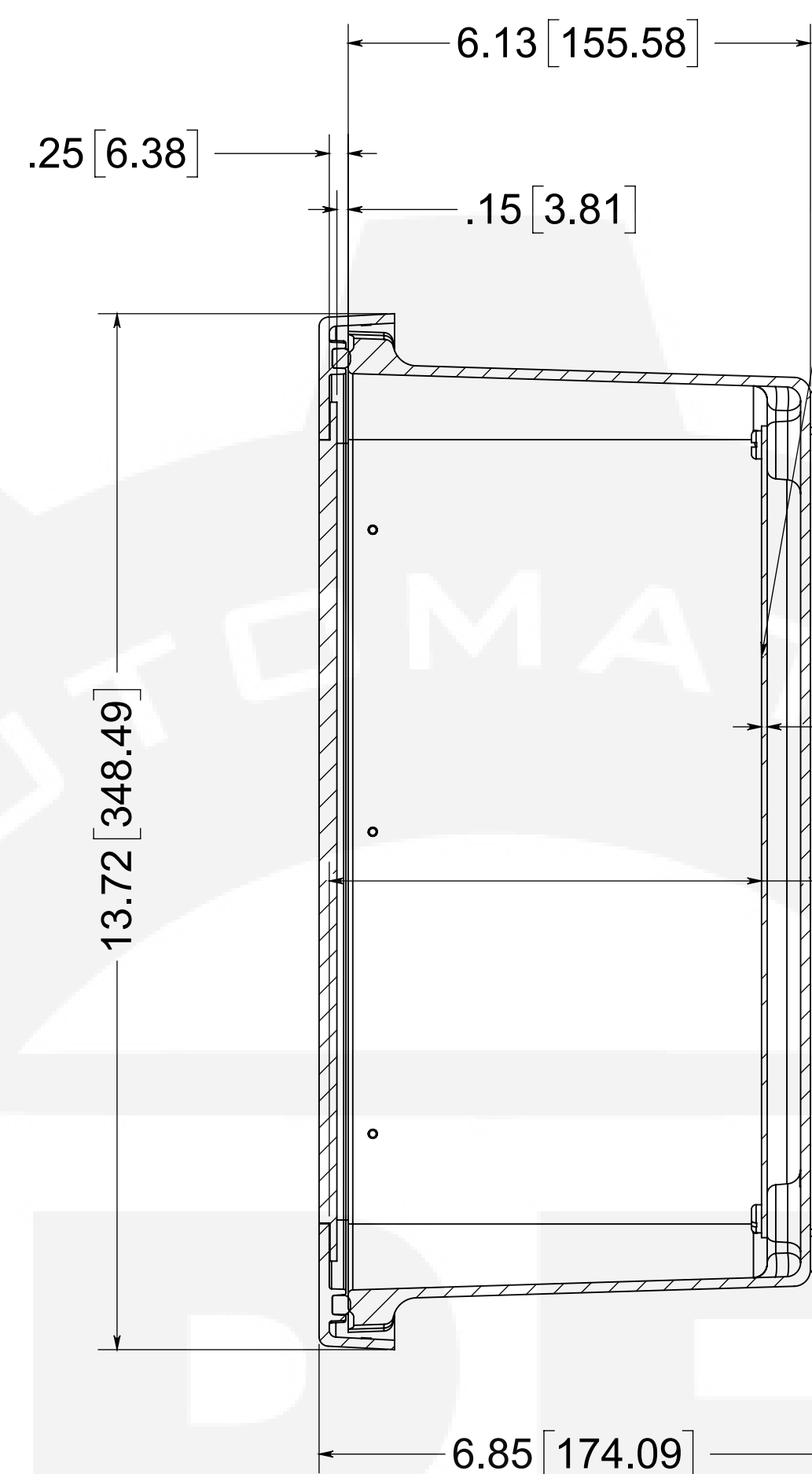
SECTION B-B
