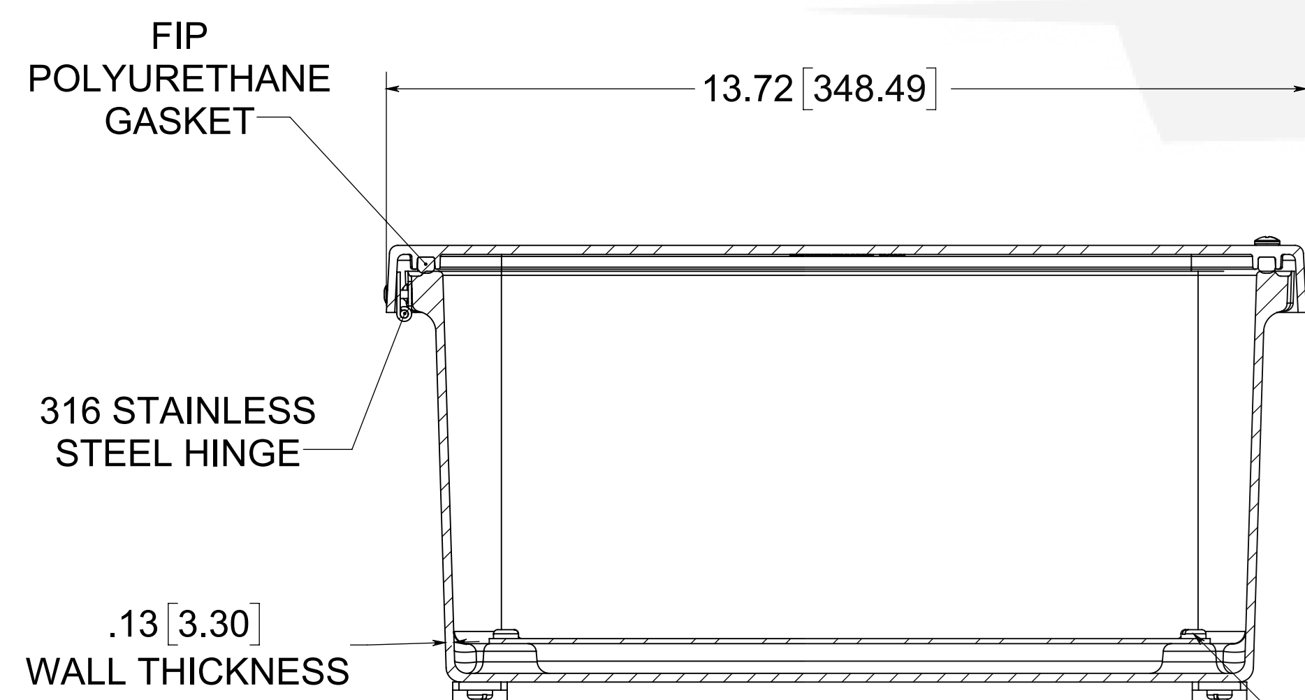
SECTION B-B
