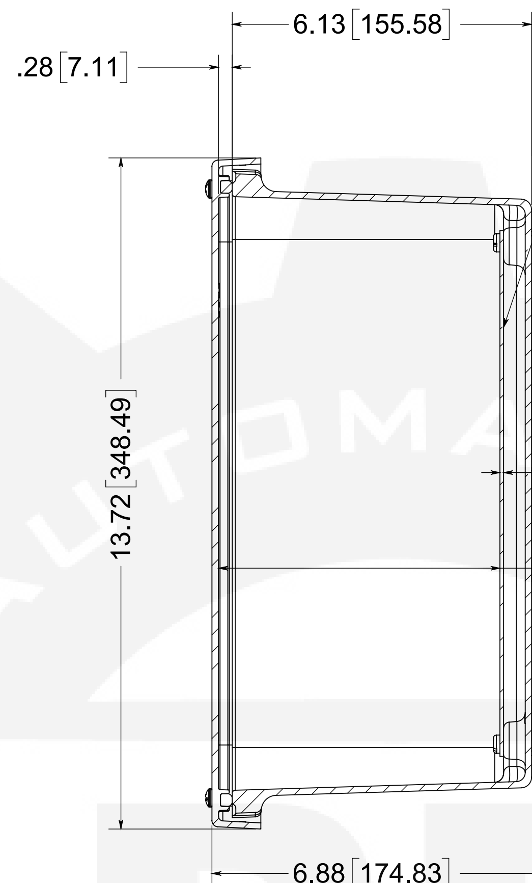
SECTION B-B
