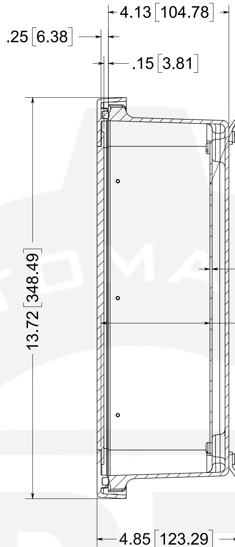
SECTION B-B
