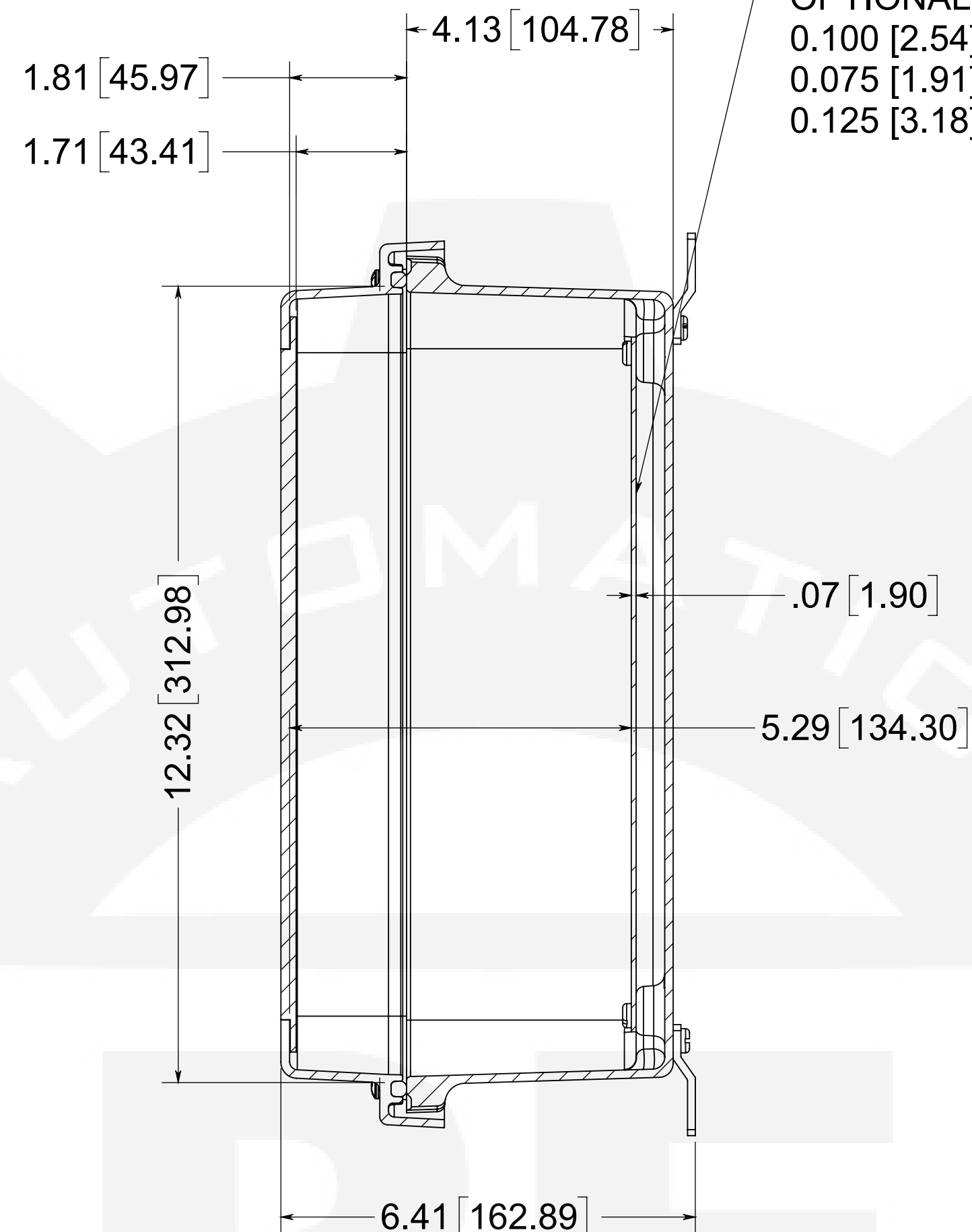
SECTION B-B
