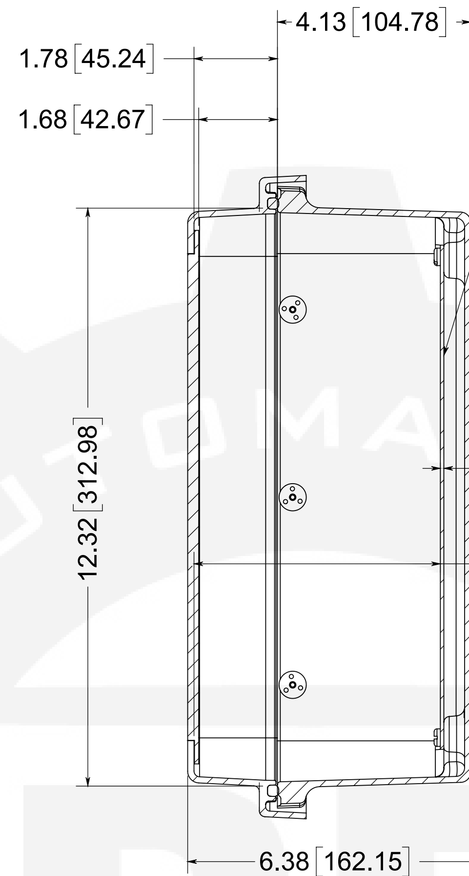
SECTION B-B
