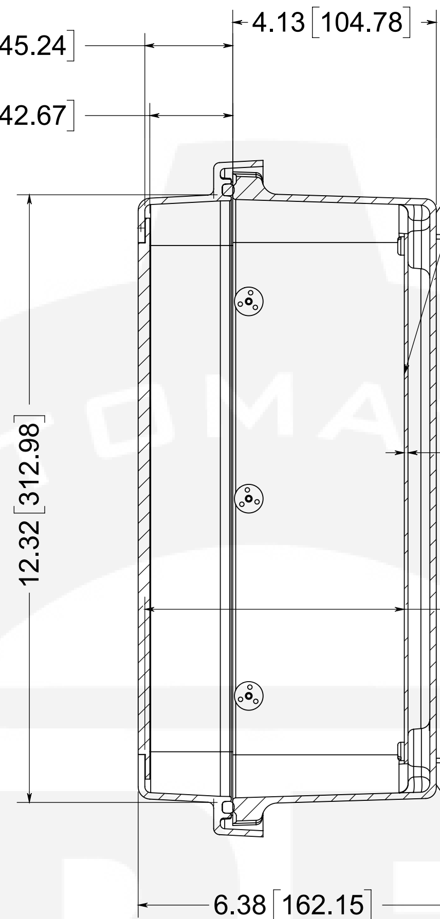
SECTION B-B
