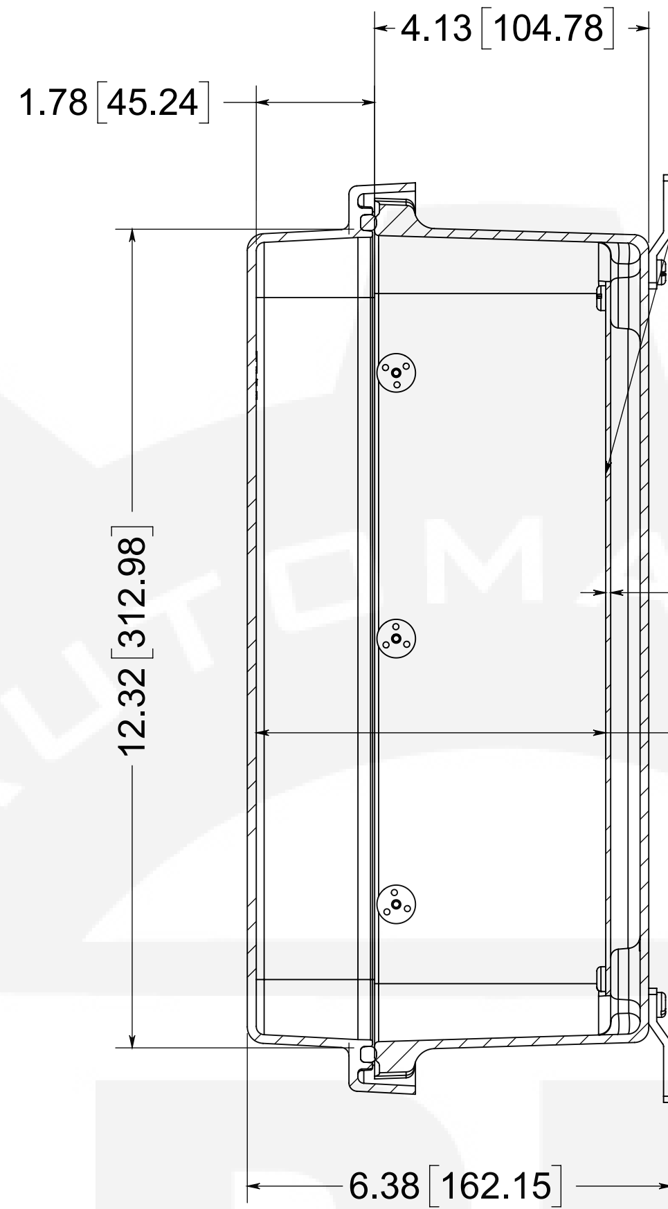
SECTION B-B
