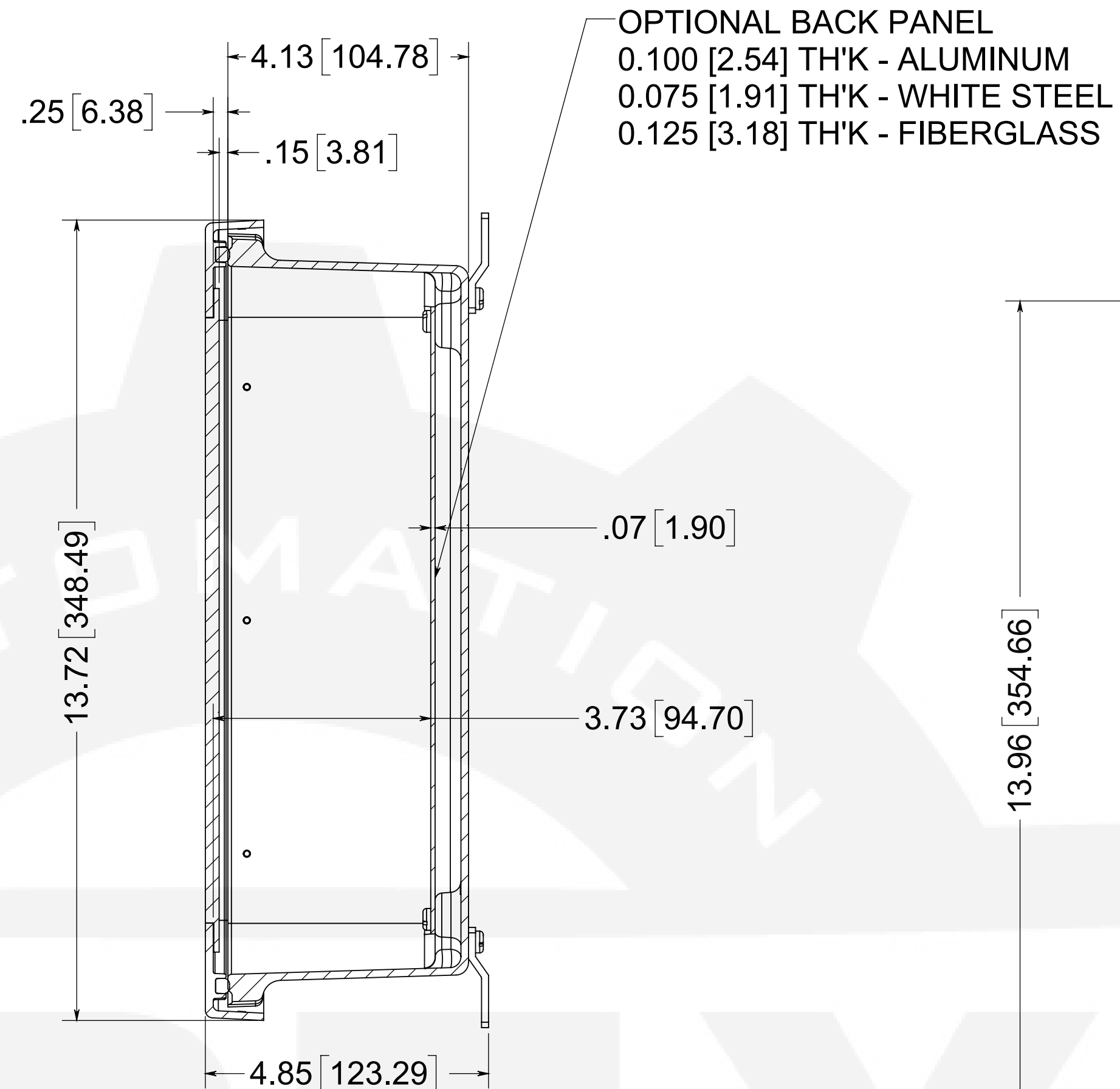
SECTION B-B
